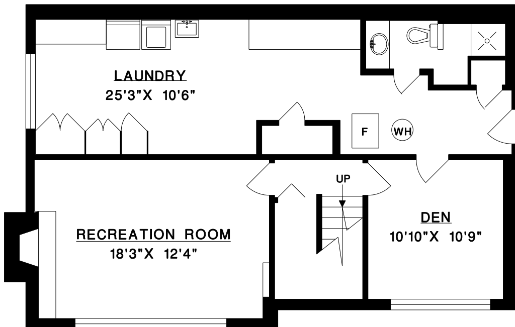
LOWER FLOOR
