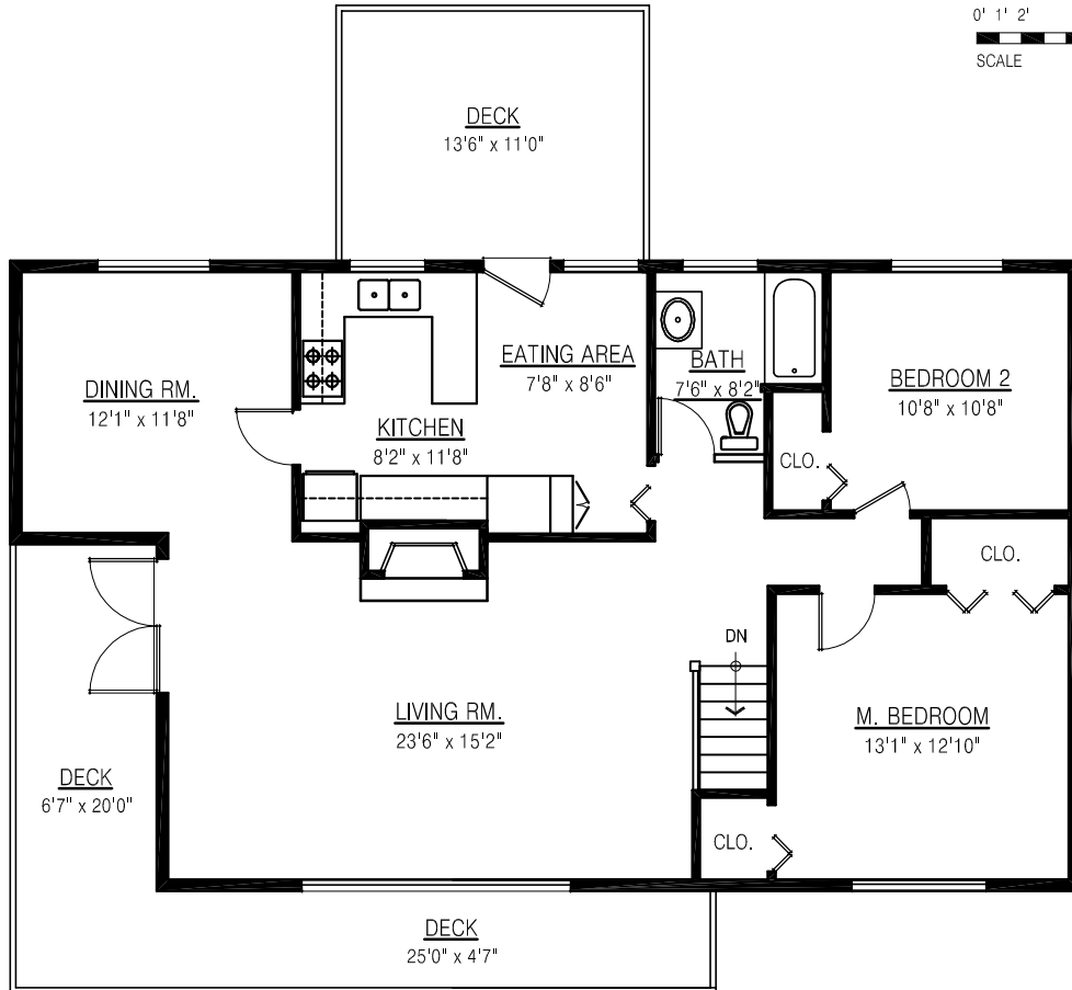
MAIN FLOOR PLAN FLOOR AREA: 1,246 sq. ft.
